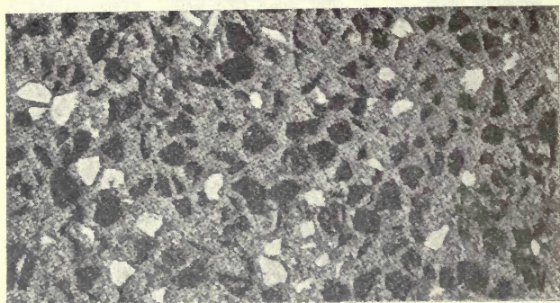
FIG. 72—SCRUBBED FACING OF 1 PART \frac{3}{4} -IN. WHITE MARBLE CHIPS, 4 PARTS \frac{3}{4} -IN. GREEN MARBLE CHIPS, 2\frac{1}{2} PARTS SAND, 1 PART CEMENT—VULCANITE PORTLAND CEMENT CO.
